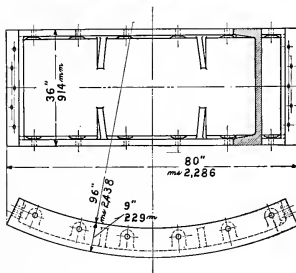
Fig. 13. Tunnel Segment Casting weighing 1500 pounds, used in making tunnel linings for the New York subway system.
